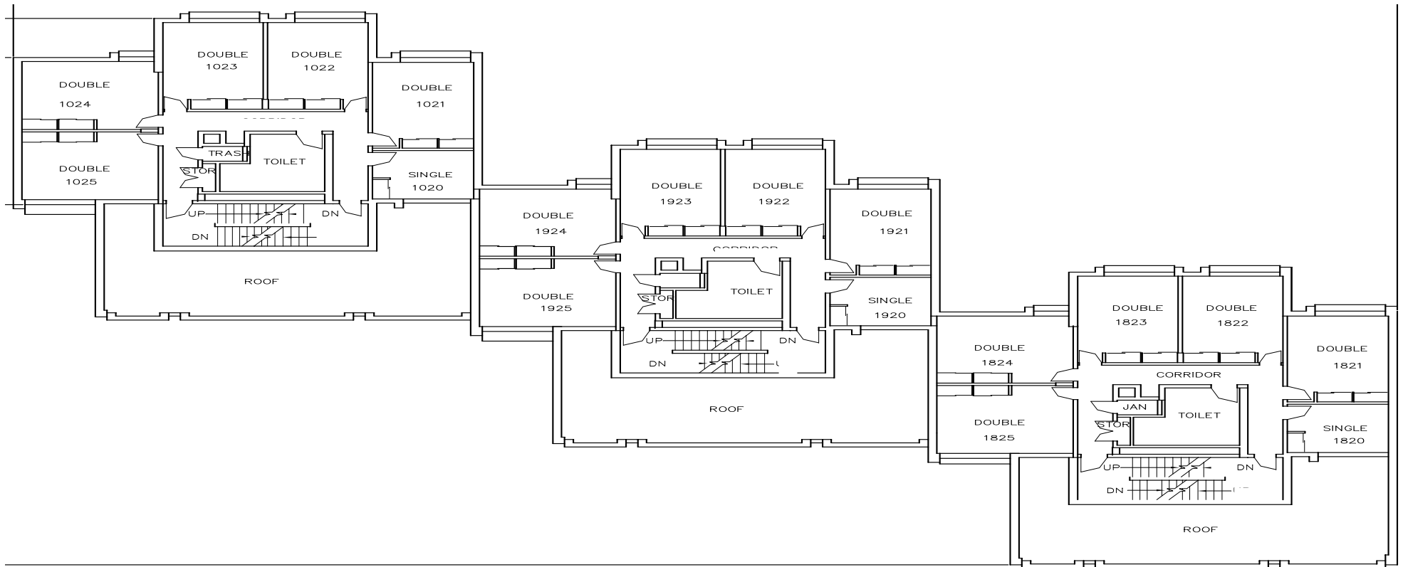
SECOND/THIRD FLOOR QUAD 1 HOUSE 10, 18-19 RUTGERS UNIVERSITY
