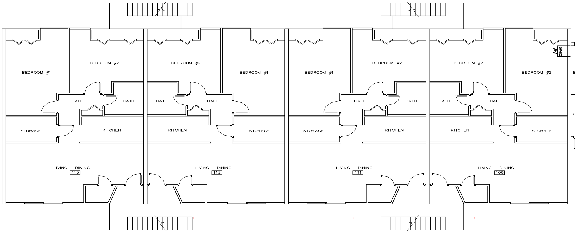
FIRST FLOOR MARVIN APTS. 109-120 RUTGERS UNIVERSITY
